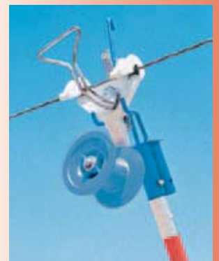
Double End Wire Raising Tool 18110812
